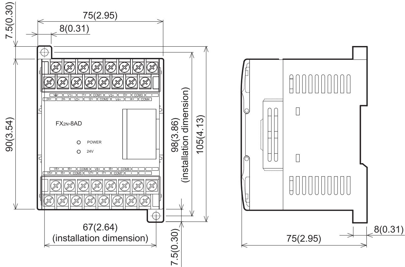
Figure 2.1: External Dimensions
