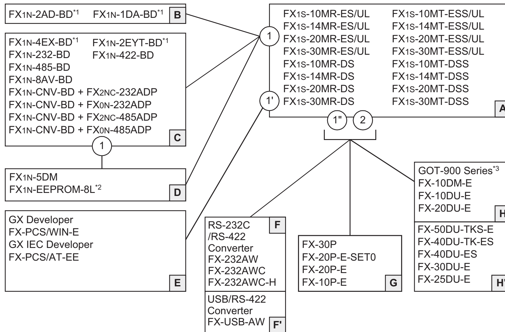
Figure 1.2: Schematic System
