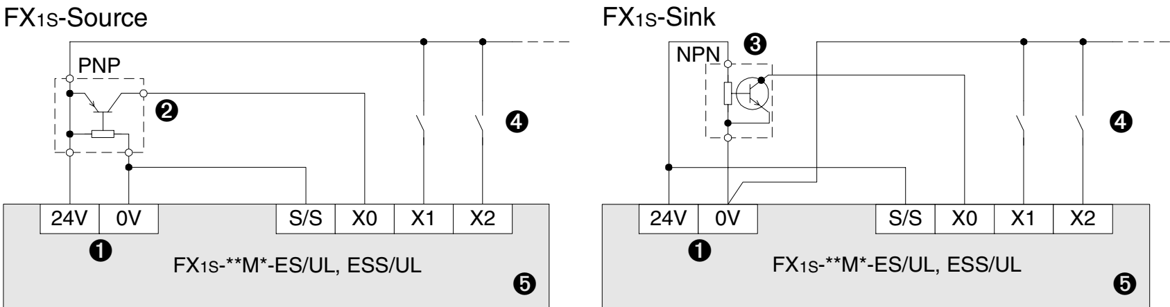
Figure 5.1: Input Wiring Diagrams
