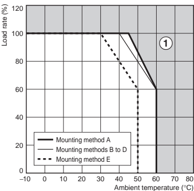
Open-frame Models and Models with Chassis: 75 W
