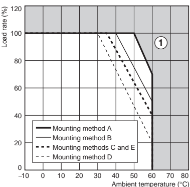
Open-frame Models and Models with Chassis: 100W
