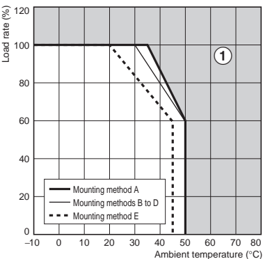
Models with Chassis and Cover: 75 W
