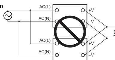
Parallel Operation Incorrect
