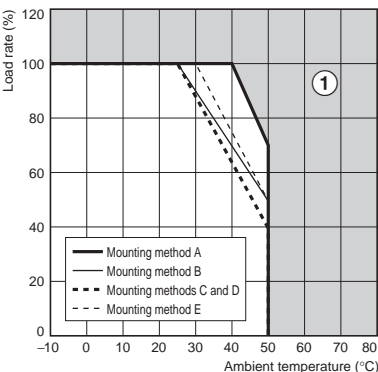
Models with Chassis and Cover: 100W
