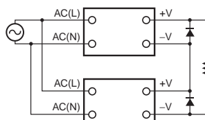
Series Operation Correct
