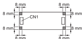
Locations of Mounting Holes on Open-frame Models
