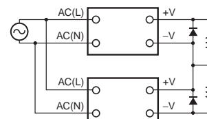
Output Voltage ( \pm ) Correct
