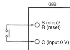
Operates with relay ON
