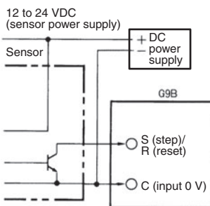
Operates with transistor ON
