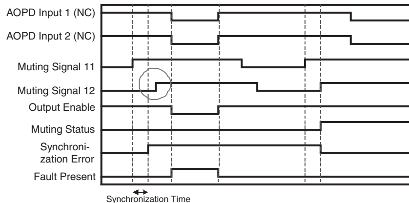
Synchronization Error (Muting Mode: Parallel Muting with 2 Sensors)
