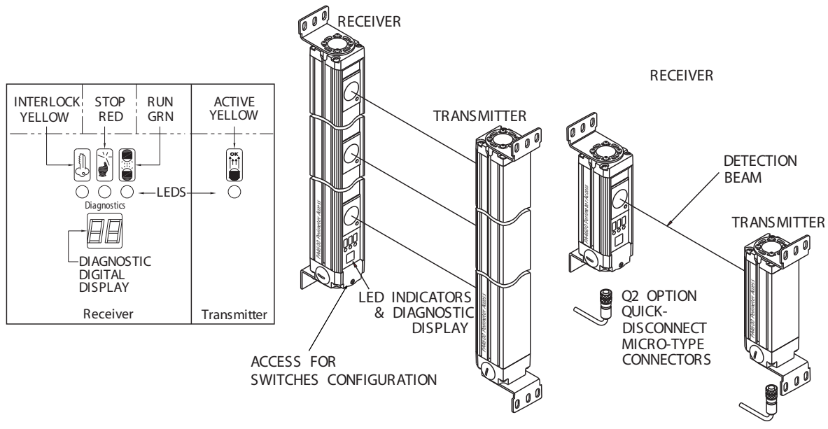
Figure 3-1 PA4600 Mechanical Drawing
