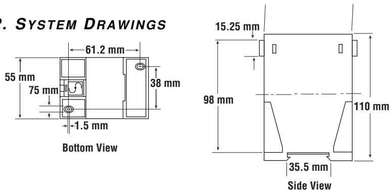
Figure 9-1 Mat Controller MC3 Dimensional Drawing
