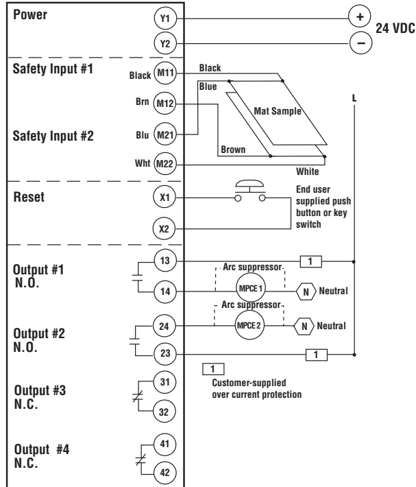
Figure 6-1 Two Normally Open Preferred Connection
