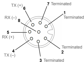
Connector B (Ethernet) M12 8-pin Socket
